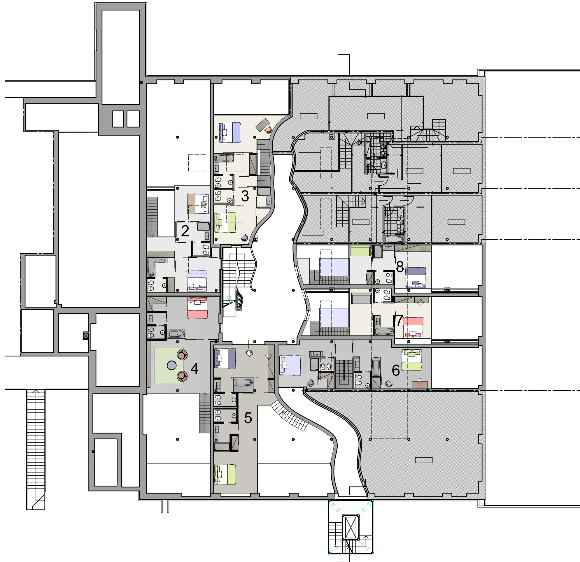
PIANO SOPPALCO
